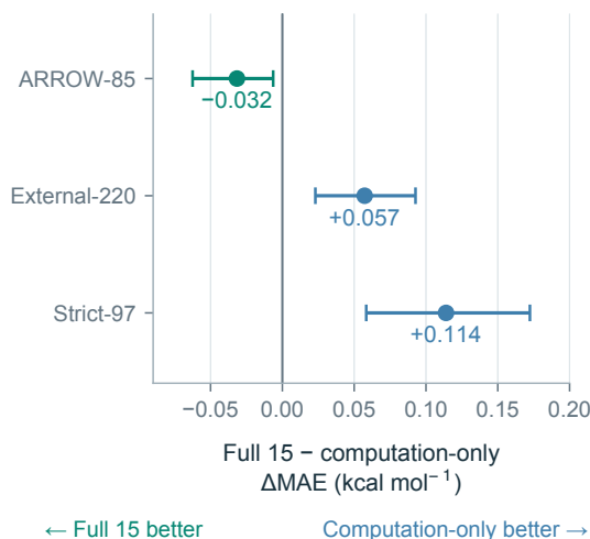
Figure 7: The preferred source composition changes with evaluation chemistry. a, The computation-only control removes five Abraham descriptors and both experimental residual corrections, \delta , while retaining the underlying OpenFF and GBn2 physical-energy predictions. The resulting computation-only set contains ten descriptors. Both models retain the same structural features, experimental endpoint labels, weights and learner. Each tile denotes one descriptor, not its magnitude. b, Absolute MAEs for structural features, all 15 responses and the ten-response control on all three reported evaluation sets. c, Paired full-minus-computation-only MAE differences with 95% intervals from 100,000 molecule resamples. Negative values favor the full model on ARROW-85; positive values favor computation-only responses externally. The strict 97 are nested within the external 220. The external extension is retrospective and compares two fixed configurations without retuning on external errors. The reversal identifies a dependence on source composition and chemistry, not one uniformly optimal response set.
