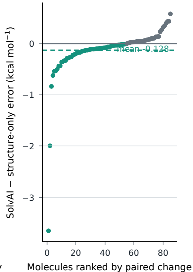
c No ARROW labels in training
