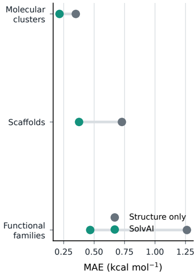
a Globally separated chemistry
