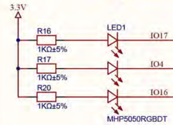
LED-RGB
