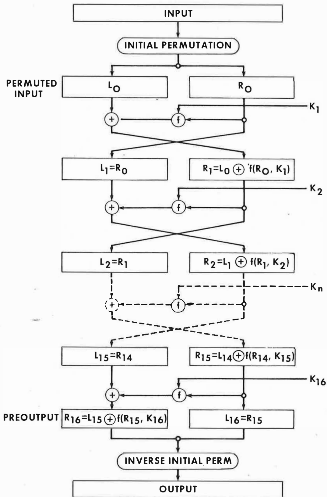
FIGURE 1. Enciphering computation.
