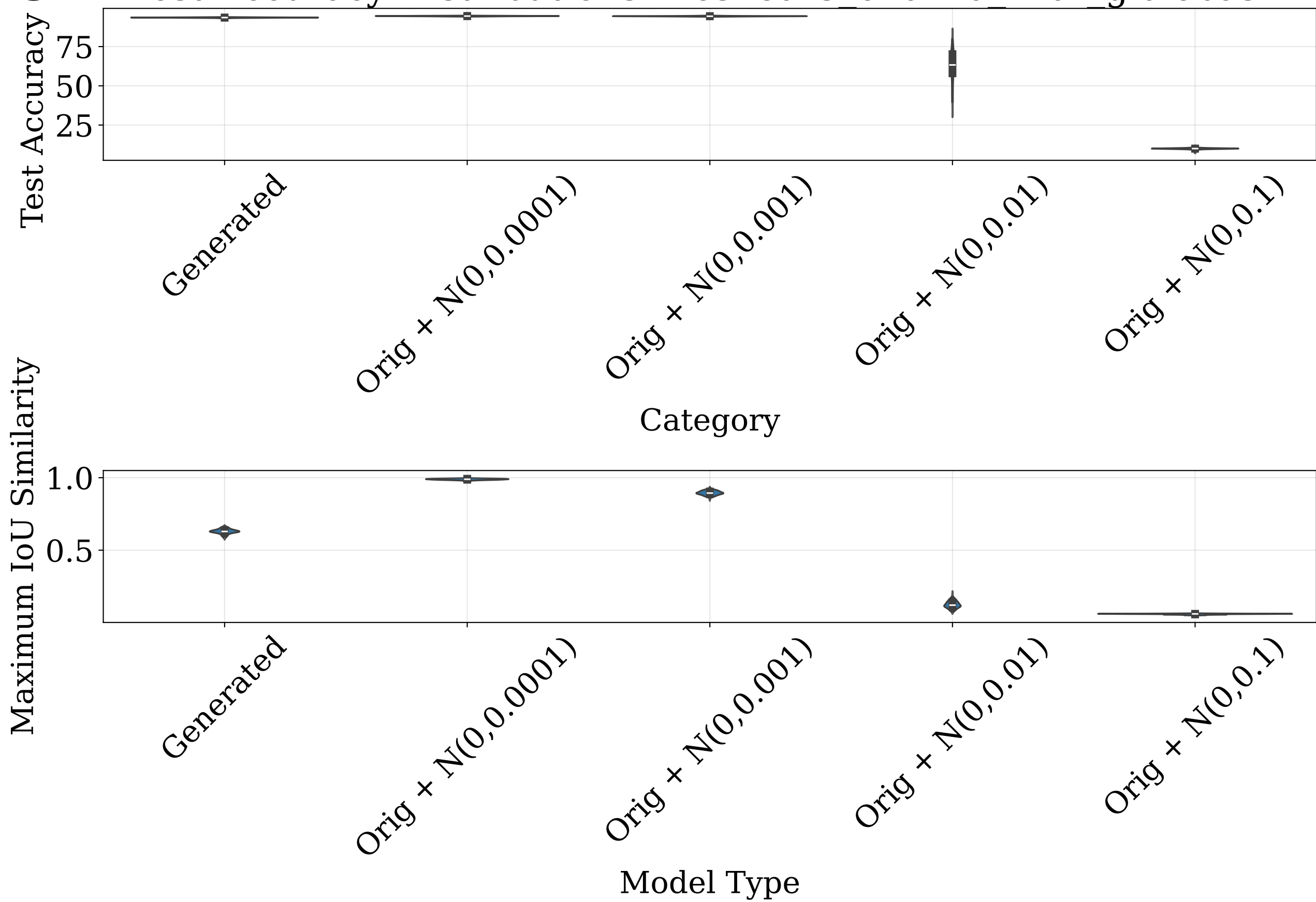
Test Accuracy Distributions - resnet18 cifar10 with_gitrebasin
