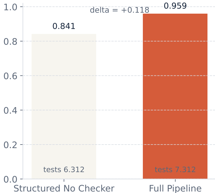
Checker score
