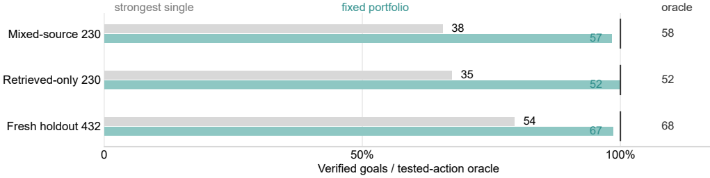
Figure 2: Result ladder. Bars are normalized within each setting by the tested-action oracle. Across the mechanism matrix, deployability anchor, and frozen holdout, the fixed typed portfolio recovers most tested oracle headroom rather than merely improving on a weak singleton baseline.
