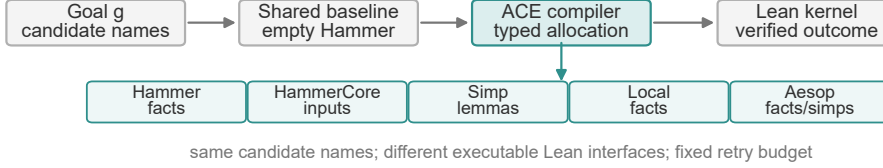
Figure 1: ACE evaluates action-conditional evidence allocation under a fixed retry budget. Selected names are compiled into typed Lean interfaces, and each routed action is checked by the Lean kernel.
