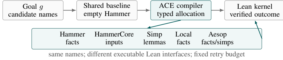
Figure 1: ACE evaluates action-conditional evidence allocation under a fixed retry budget. Selected names are compiled into typed Lean interfaces, and each routed action is checked by the Lean kernel.
