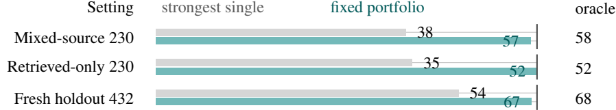
Figure 2: Result ladder. Bars are normalized within each setting by the tested-action oracle. Across the mechanism matrix, deployability anchor, and frozen holdout, the fixed typed portfolio recovers most tested oracle headroom rather than merely improving on a weak singleton baseline.
