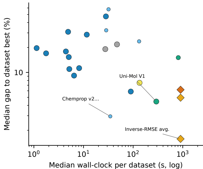
a Regression
