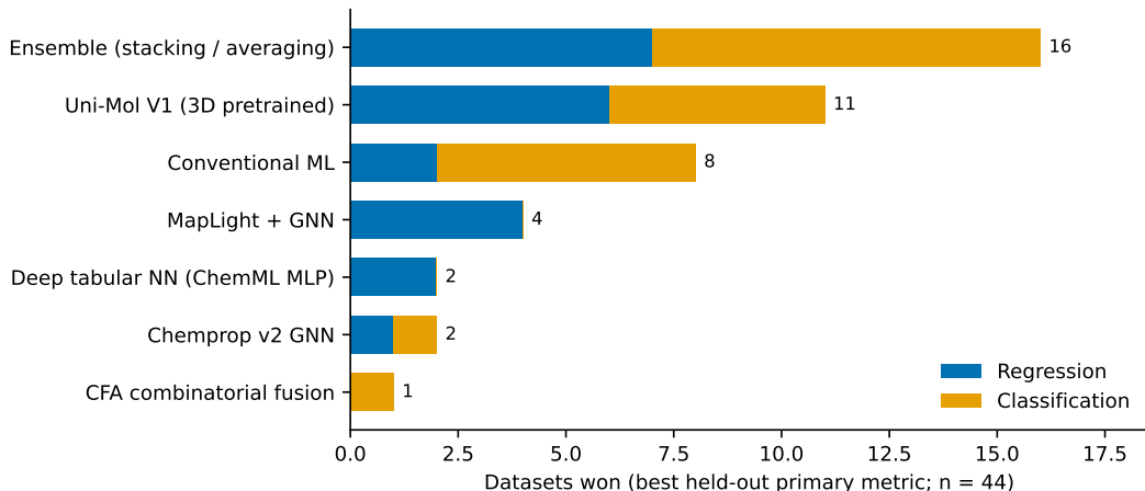
Figure 2: Datasets won by each architecture family, split by task kind. A win is the best held-out primary metric on that dataset among all 28 models. Single split and single seed: individual placements are provisional and no variance is estimated (see Limitations).
