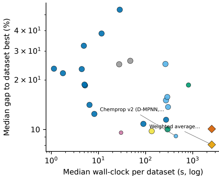
a Regression
