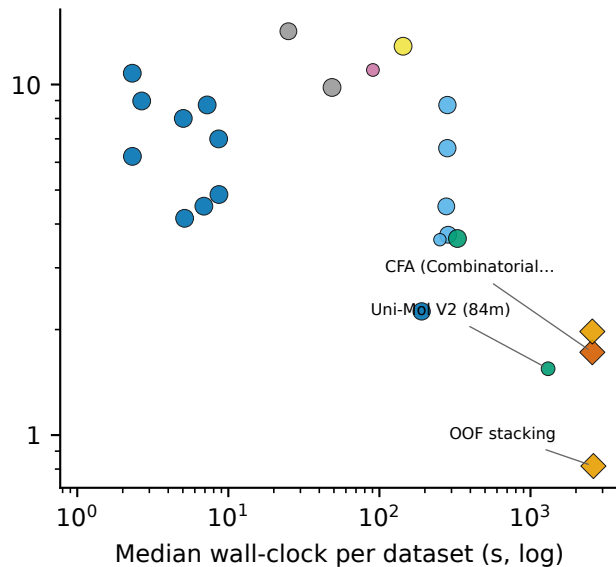
b Classification
