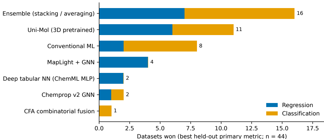
Figure 2: Datasets won by each model family, split by task kind. A win is the best held-out primary metric on that dataset among all 28 models. Single split and single seed: individual placements are provisional and no variance is estimated (see Limitations).
