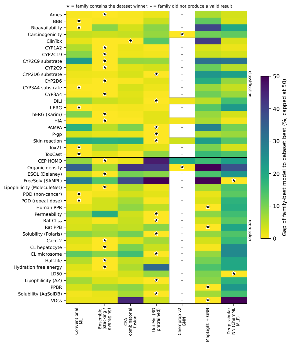
Figure 6: Relative gap of each family’s best model to the per-dataset best (% , capped at 50), for every dataset. Stars mark the family containing the dataset winner; dashes mark families that produced no valid result for that dataset. Classification datasets are shown above the rule, regression below.
