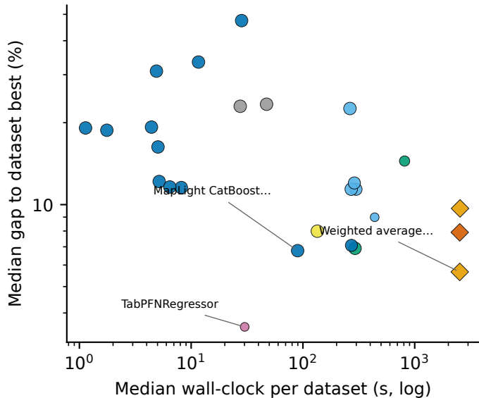
a Regression
