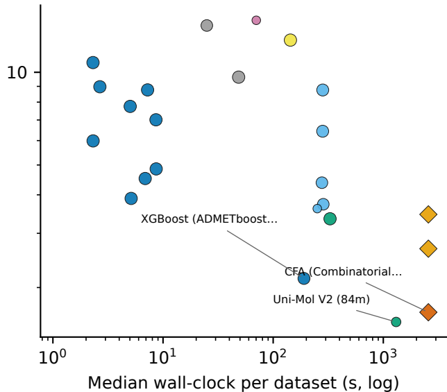
b Classification
