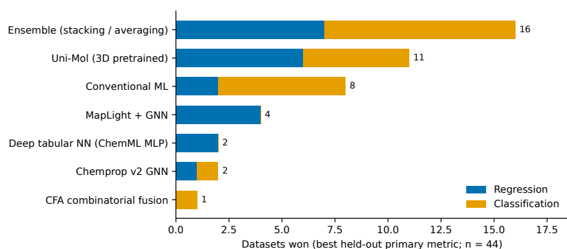
Fig. 3 Datasets won by each model family, split by task kind. A win is the best held-out primary metric on that dataset among all 31 models. Single split and single seed: individual placements are provisional and no variance is estimated (see Limitations).
