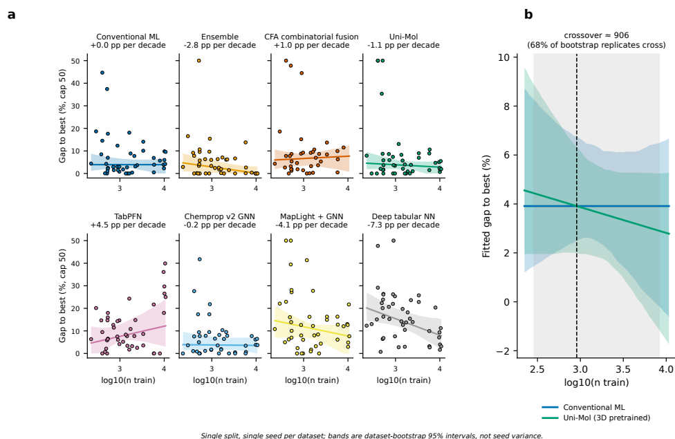
Fig. 8 (a) Relative gap of each family's best model to the per-dataset best versus \log_{10} training-set size, with Theil-Sen fits and dataset-bootstrap 95% bands (gaps capped at 50% for display). (b) Fitted gap curves for conventional ML and Uni-Mol; the dashed line and grey span mark the estimated crossover and its bootstrap CI when one exists. Single split and single seed per dataset: bands reflect dataset resampling, not seed variance.
