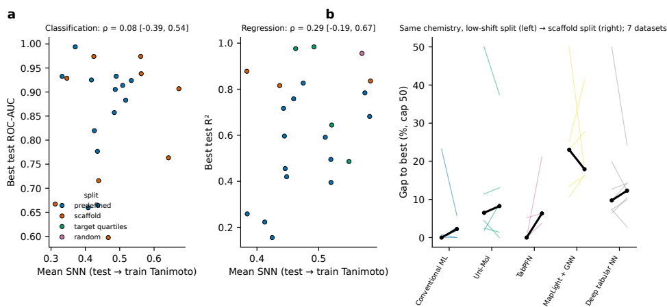
Fig. 9 (a) Achievable best held-out metric versus mean test-to-train nearest-neighbour Tanimoto (SNN), by task and split protocol. (b) Family gaps on the 7 datasets that were re-split from random or target-quartile splits to scaffold splits between the RTX 4060 and A100 runs (Section 3.10); thin lines are datasets, thick lines are medians.
