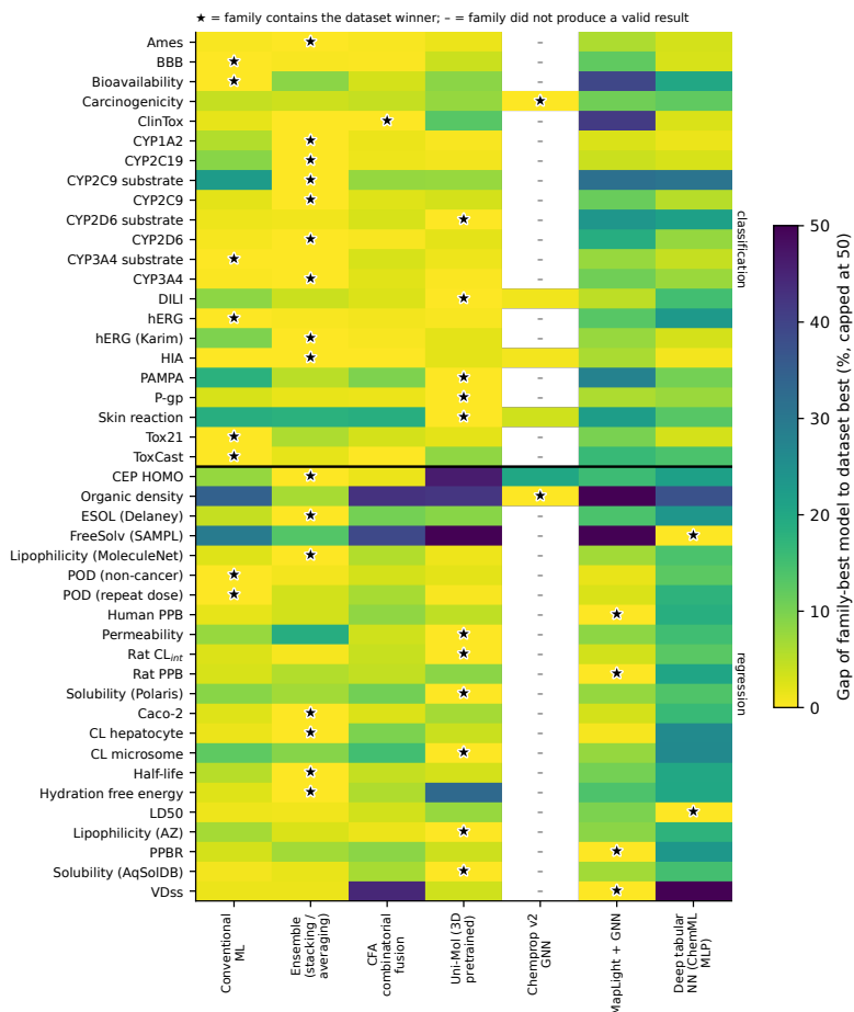
Fig. 7 Relative gap of each family’s best model to the per-dataset best (%), for every dataset. Stars mark the family containing the dataset winner; dashes mark families that produced no valid result for that dataset. Classification datasets are shown above the rule, regression below.
