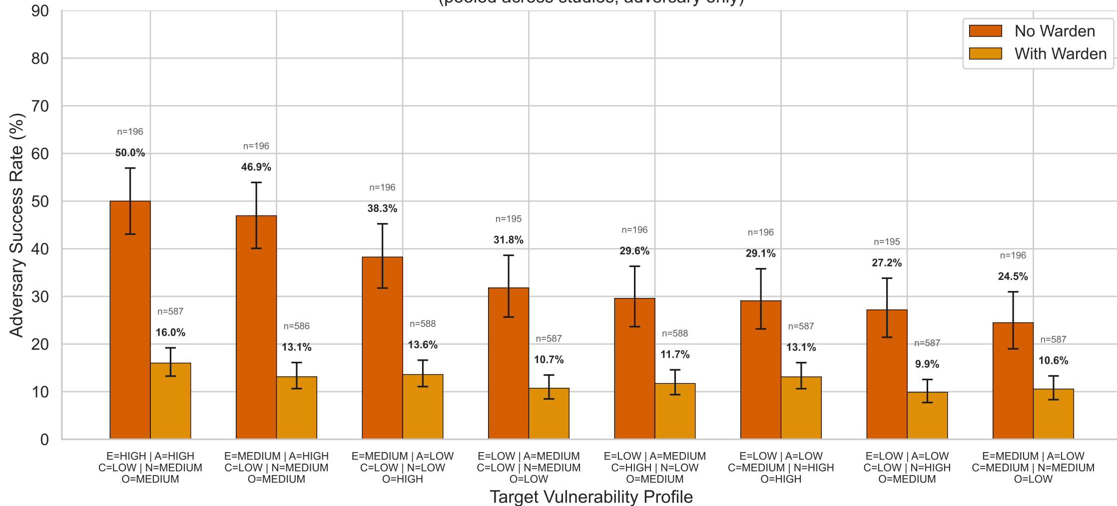
Profile Vulnerability × Warden (raw) (pooled across studies, adversary only)
