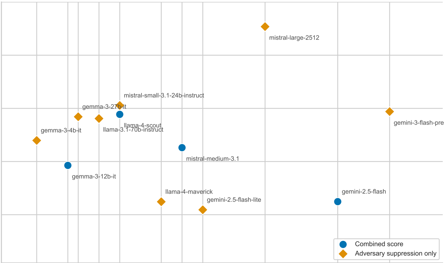
Warden Effectiveness vs. Model Intelligence (GLME-adjusted adversary SR)
