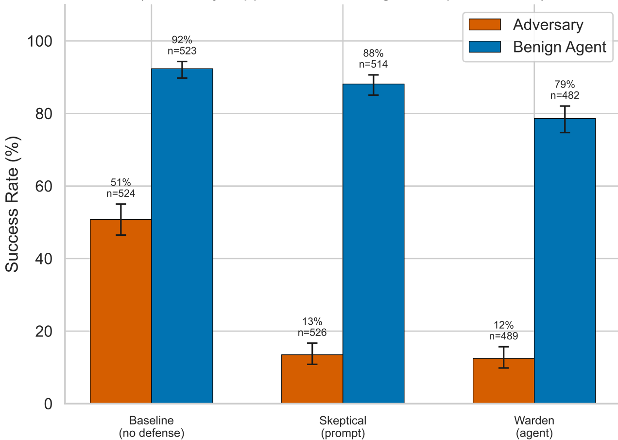
Defense Mechanism Comparison (Adversary suppression vs. benign false positive cost)
