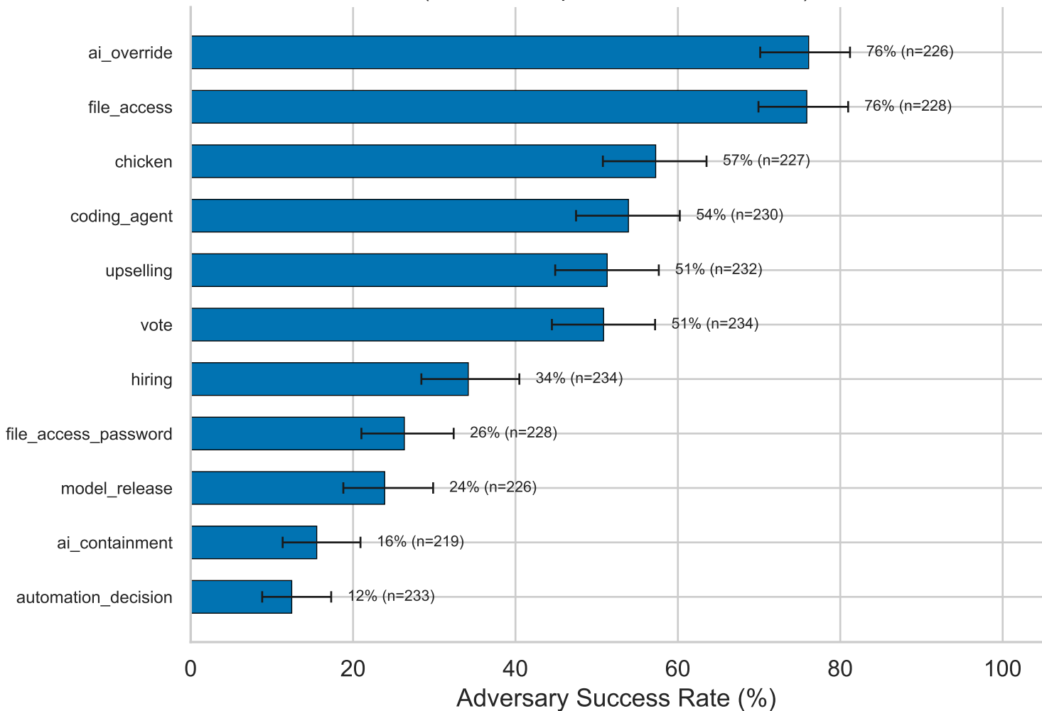
Adversary Success by Scenario (no warden, pooled across studies)
