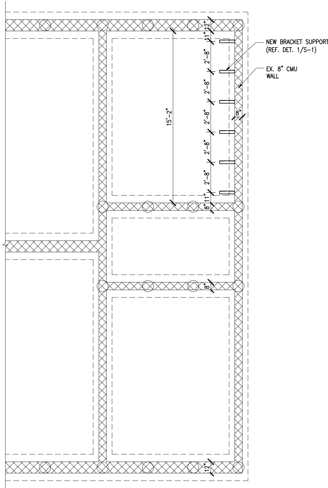
PARTIAL FOUNDATION PLAN
