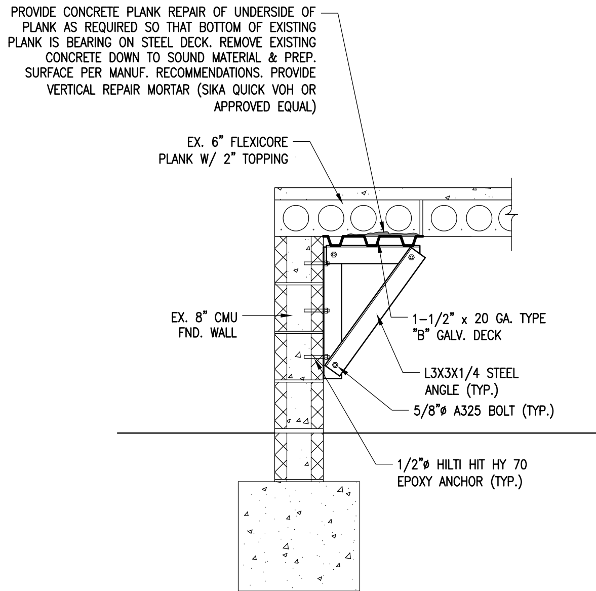
1 SUPPORT DETAIL
