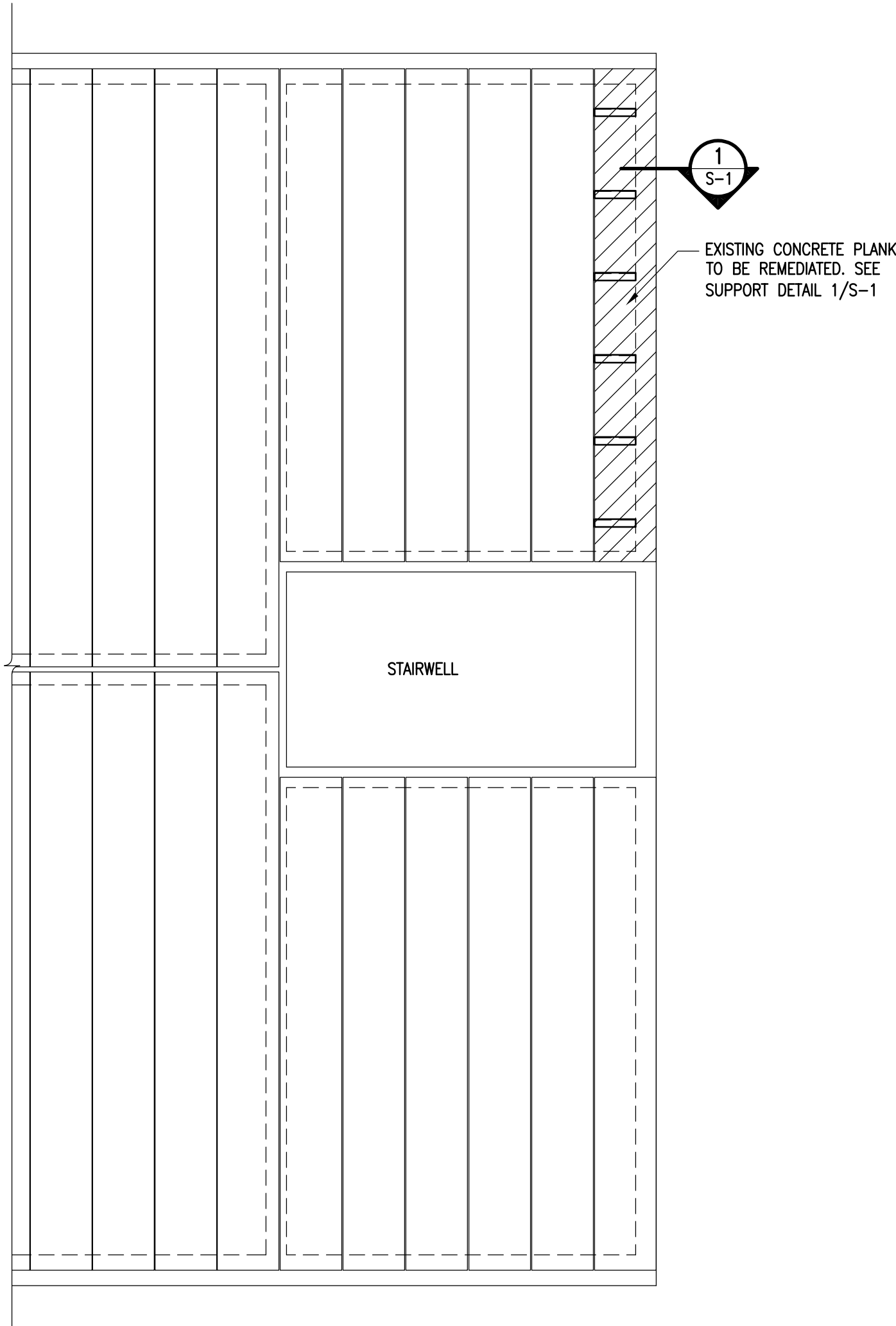
PARTIAL FIRST FLOOR FRAMING PLAN
