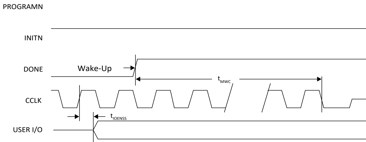
Figure 3.21. Wake-Up Timing
