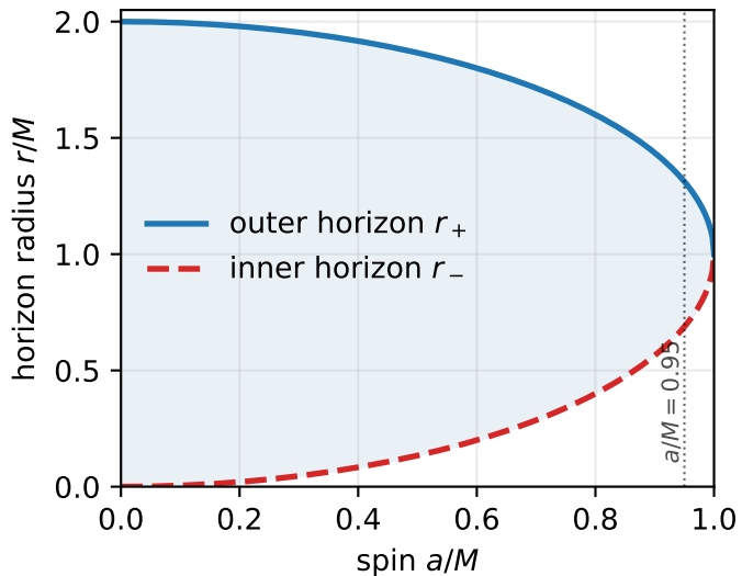
(a) Kerr horizons r_{\pm} = M \pm \sqrt{M^2 - a^2}
