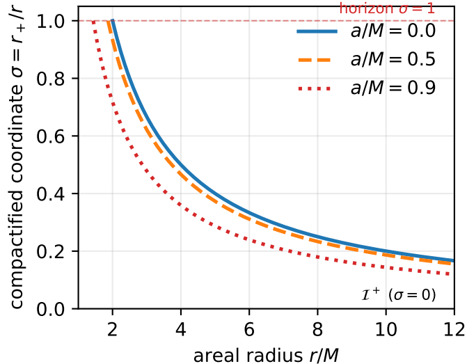
(b) Radial compactification
