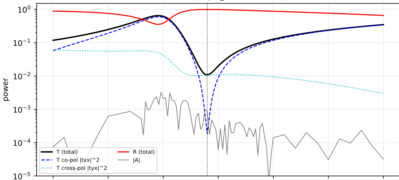
FIGURE 3 - P0750 resonance at 0.2-nm sampling: T_{\min} = 0.011 (co-pol 1.8e-4 ), R = 0.988 , A = 9e-4
