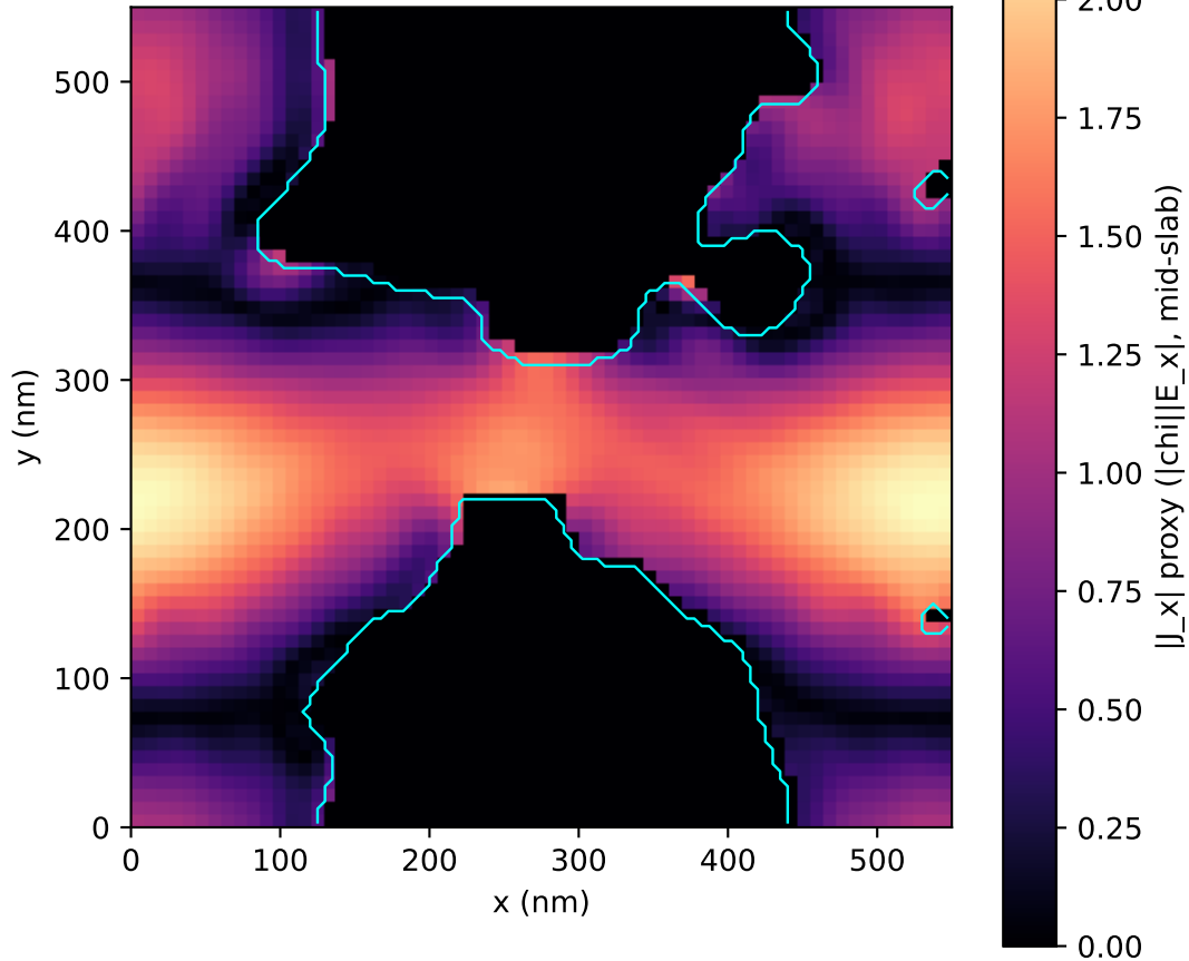
induced current at 1332.5 nm on the geometry outline (h = 250)
