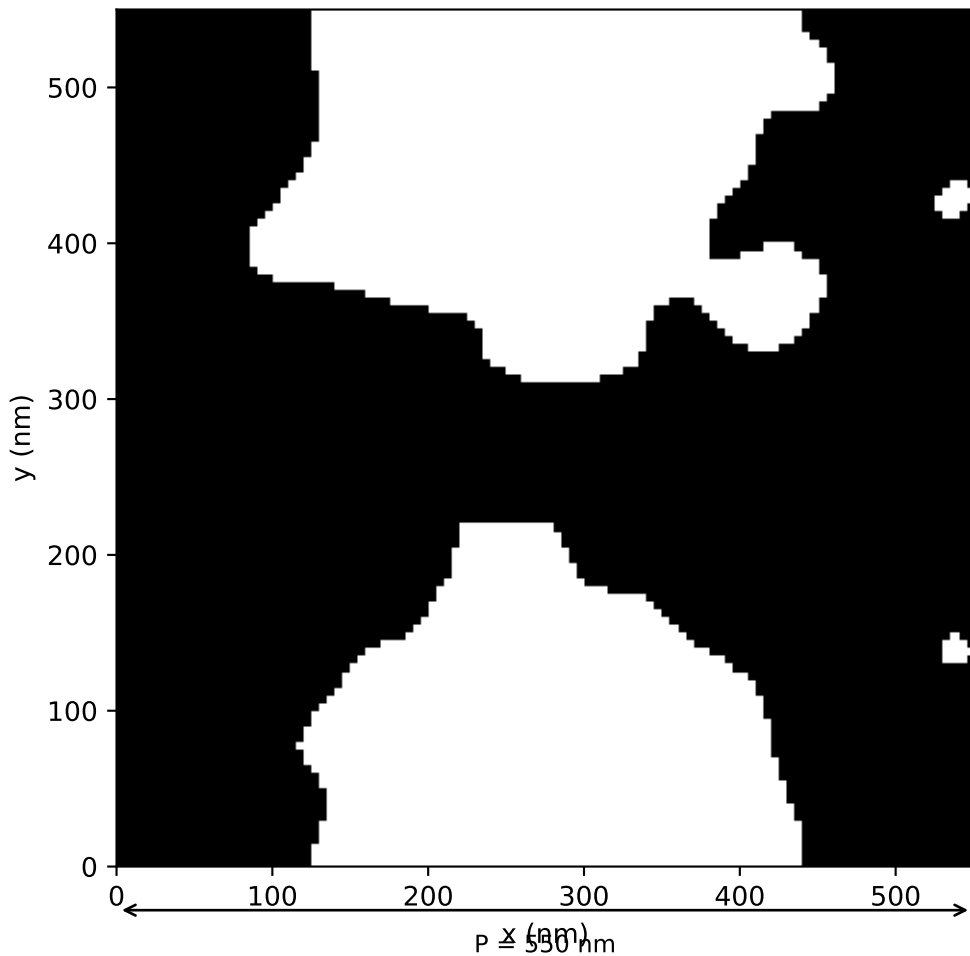
P0550_H0250_seed011 - hard-binary top view dark = a-Si (fill 0.618), white = air; P = 550 nm
