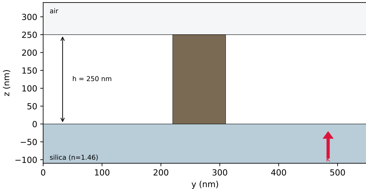
y-z cross section at x = P/2
