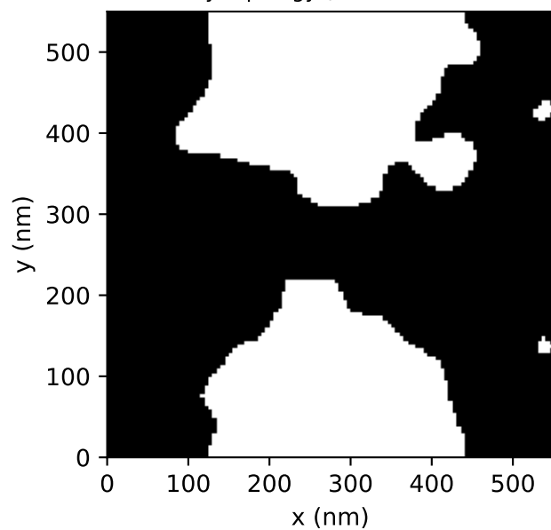
A P0550 hard-binary topology (a-Si dark, P = 550 nm, fill 0.62)
