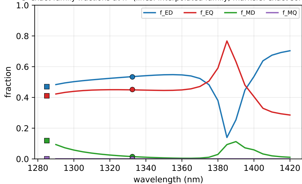
C exact family fractions at h^* (lines: interpolated family; markers: exact solves)
