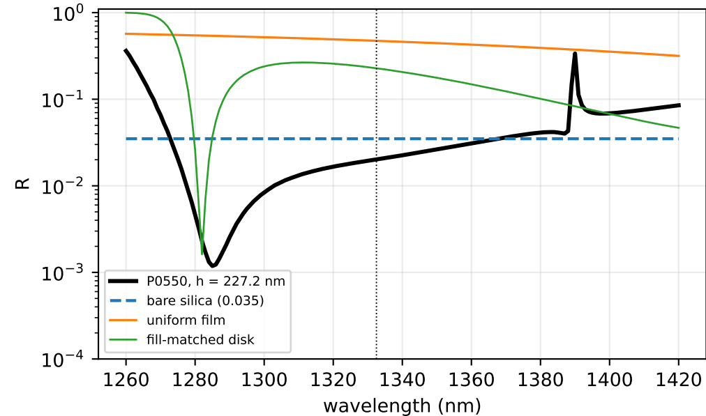
B is it antireflective? R vs all baselines
