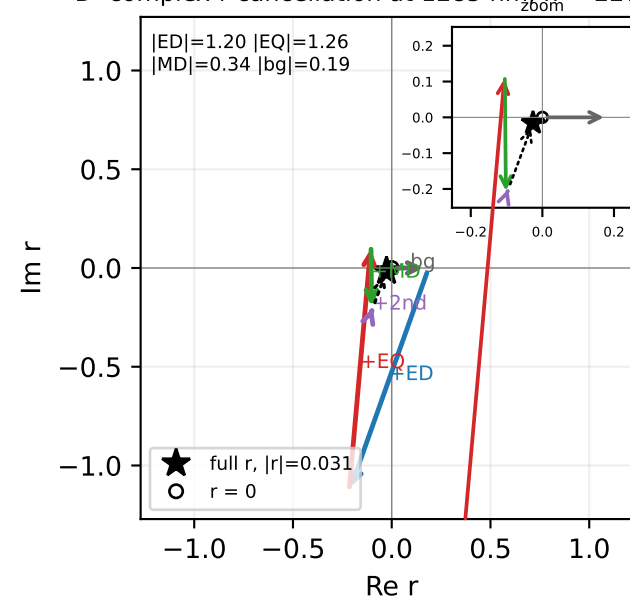
D complex-r cancellation at 1285 nm, h = 227.2 nm
