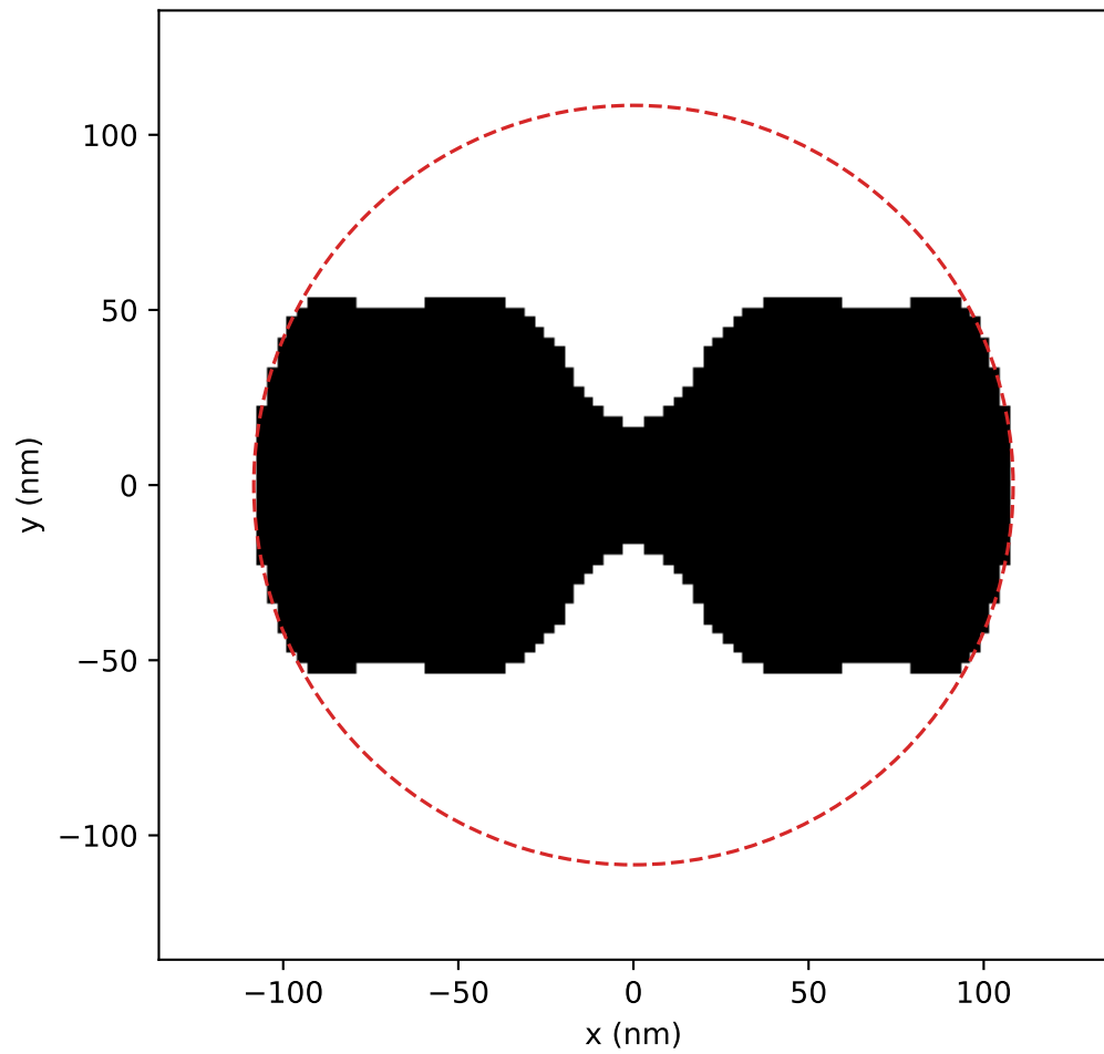
hard-binary top view + rotation-safe envelope
