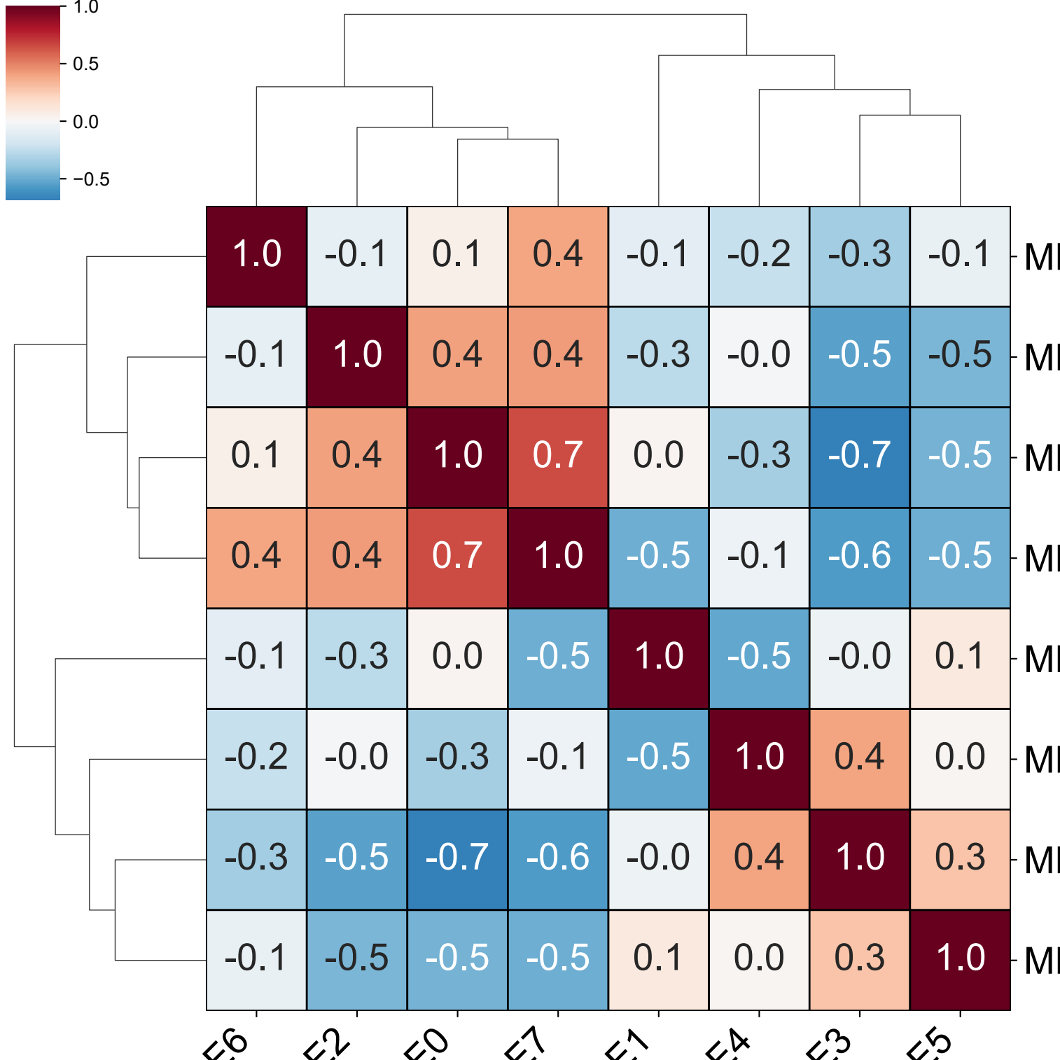
Correlation Heatmap (Partial)
