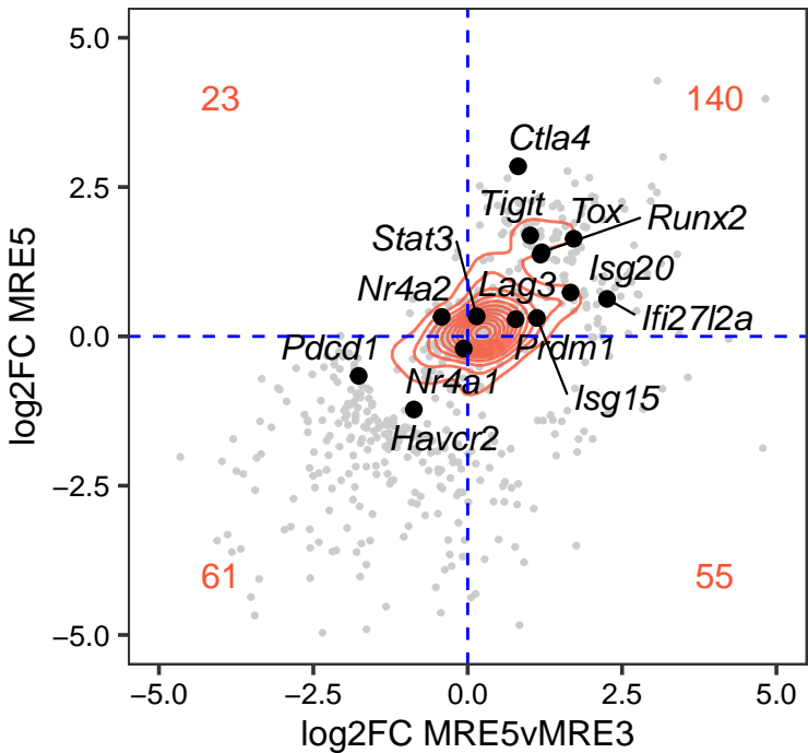
MRE5 vs MRE5vMRE3
