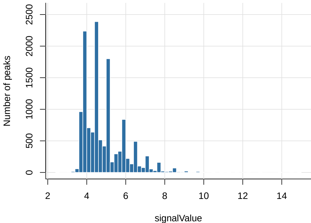
Distribution of signalValue: late_Runx3.merged.macs2_peaks
