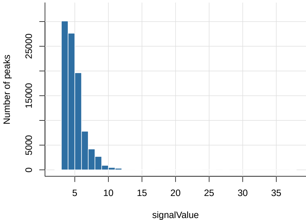
Distribution of signalValue: shRunx3_Runx1.merged.macs2_pea
