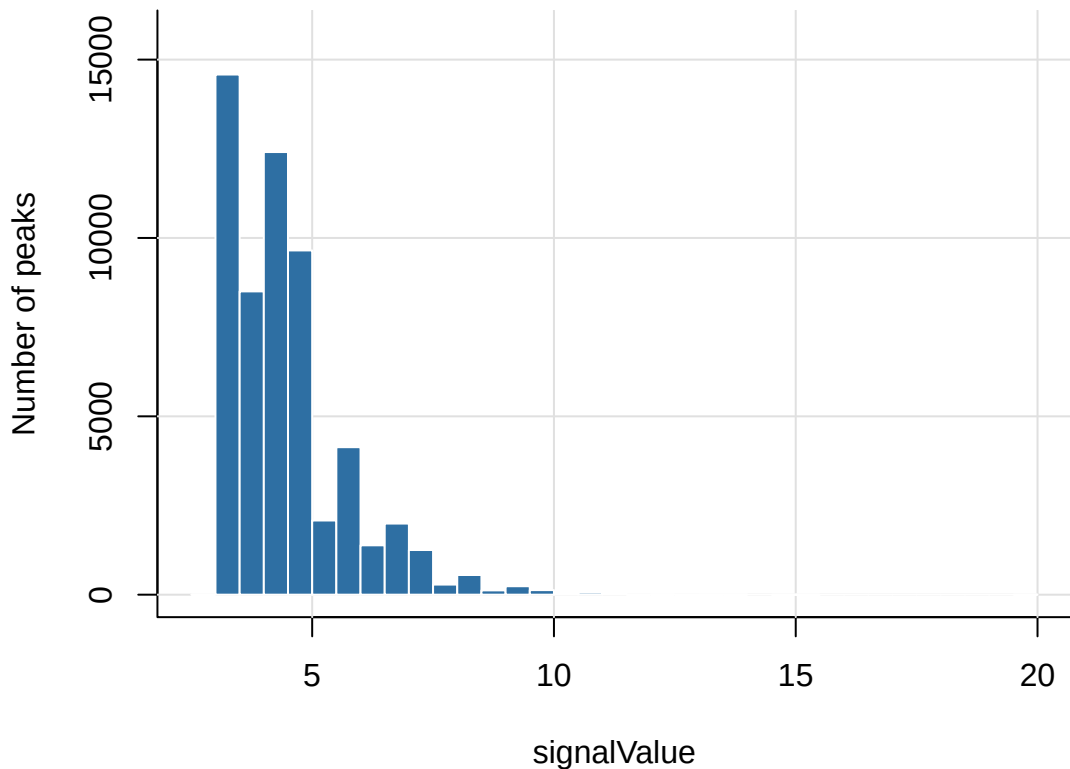
Distribution of signalValue: terminal_Runx1.merged.macs2_pea
