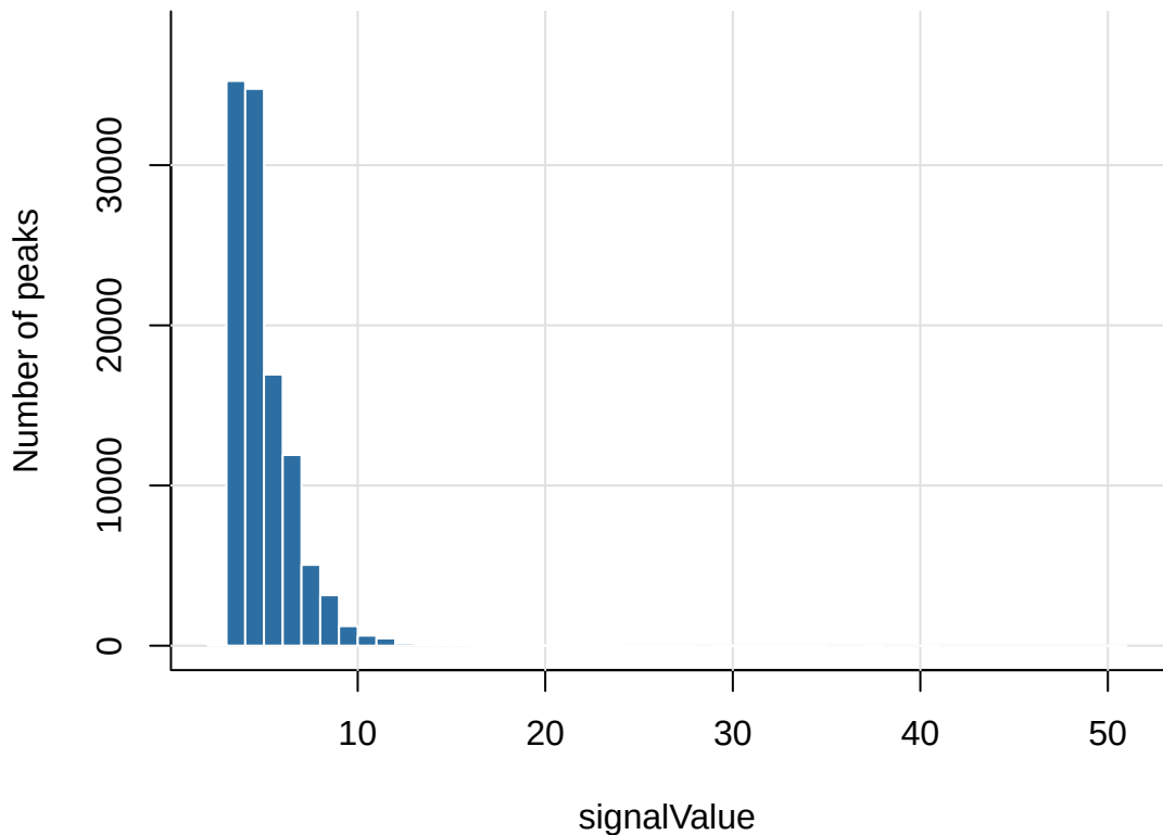
Distribution of signalValue: shRunx3_Runx3.merged.macs2_pea
