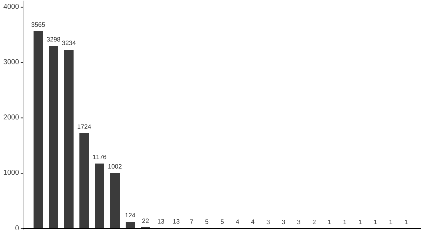
Runx1 (Stringent): Peak Intersections
