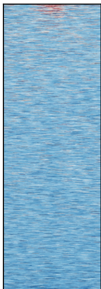
Runx1-Bound
