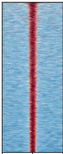
Runx1-Unknown
