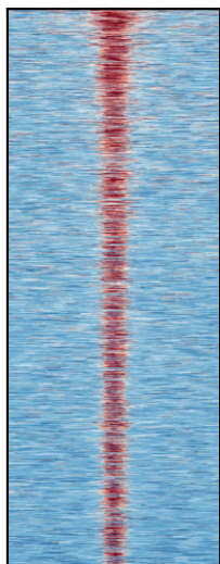
Runx1-Constant
