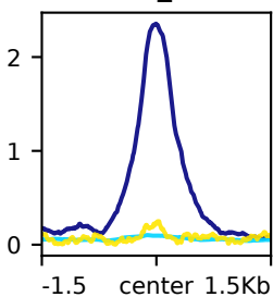
shCd19_Runx3
