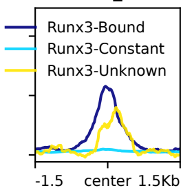
shRunx3_Runx3
