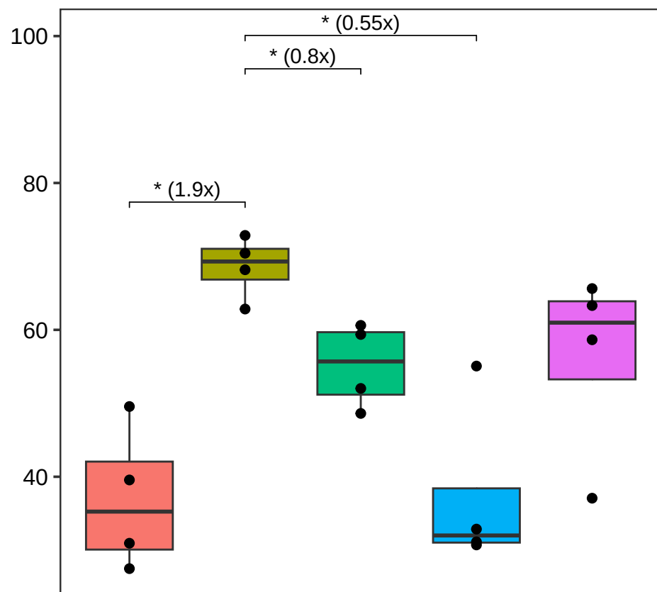
TcmL
