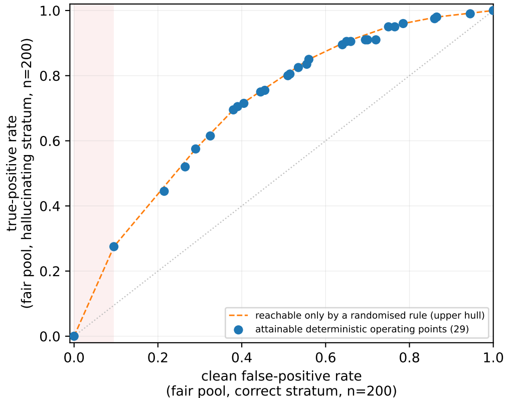
Achievable ROC: a finite point set, not a curve
