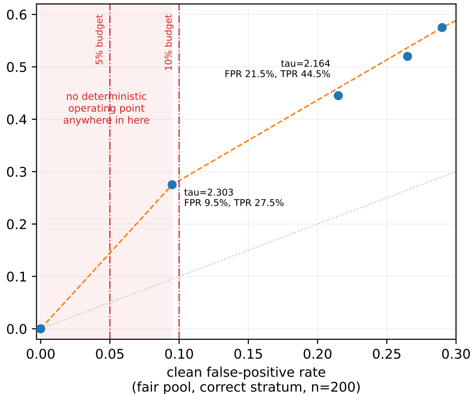
No threshold exists below FPR 9.5%
