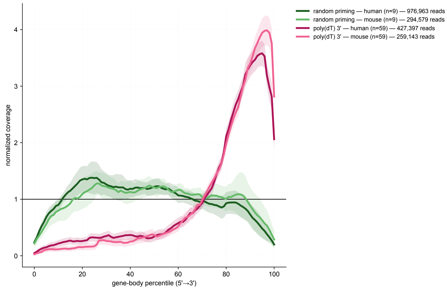
Gene-body coverage — poly(dT) 3' vs random priming, human (dark) vs mouse (light) (shaded = 95% CI of the mean) inserts ≤500 bp · ribosomal proteins removed · transcripts ≥1000 bp · ≥1000 reads/species
