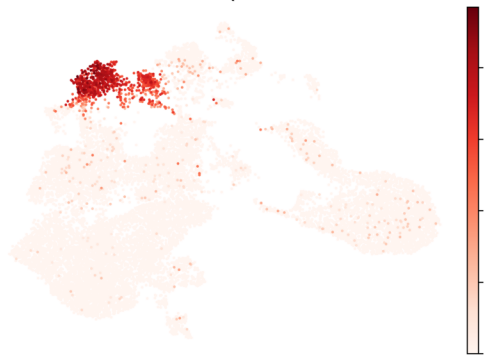
C1QB
