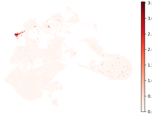
FCGR3B
