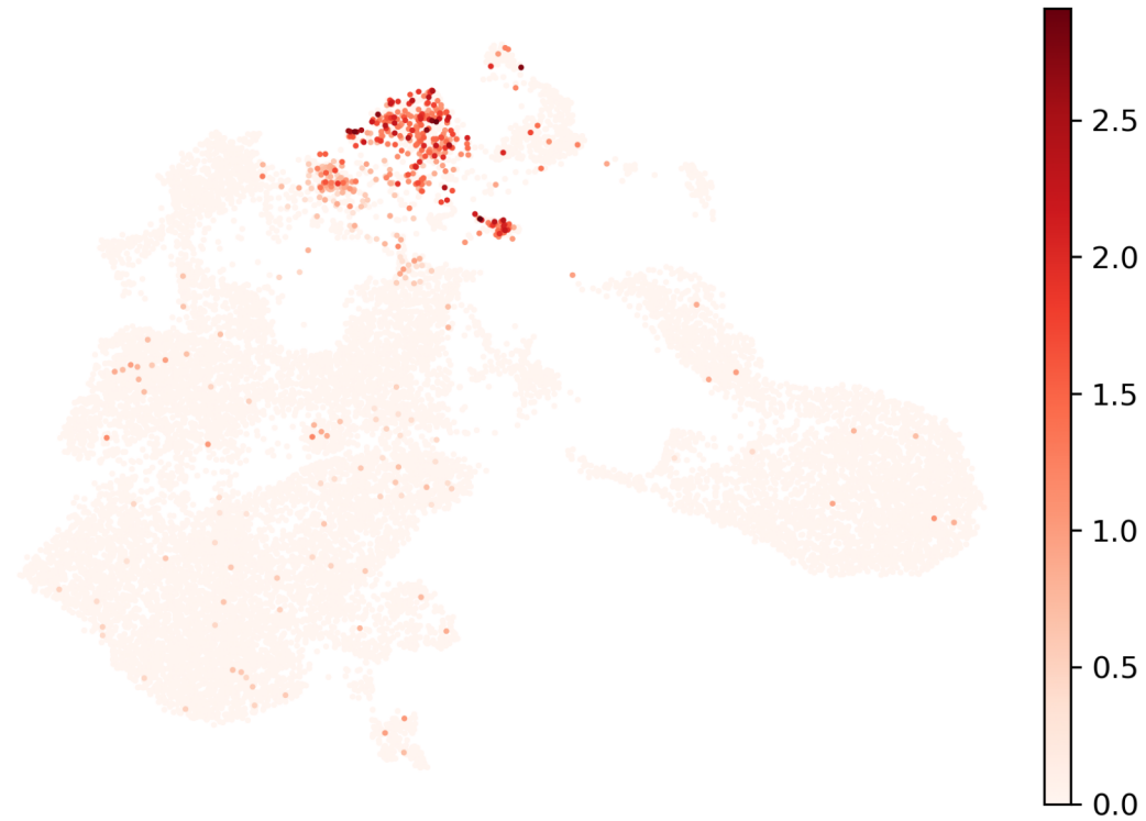
RGS5
