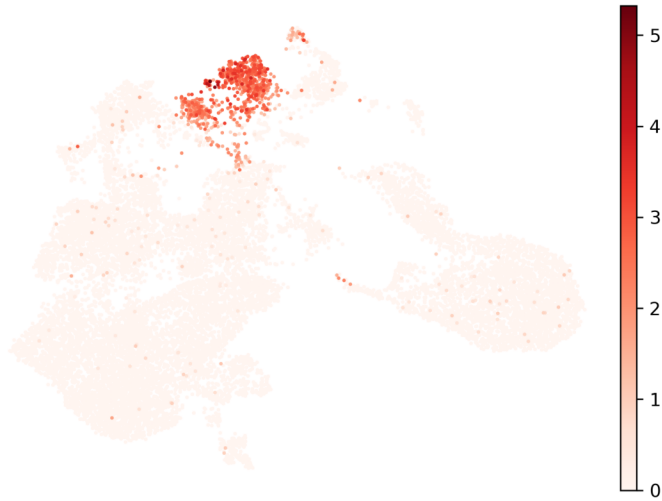
COL1A1
