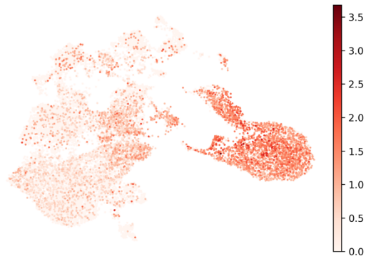
TFRC
