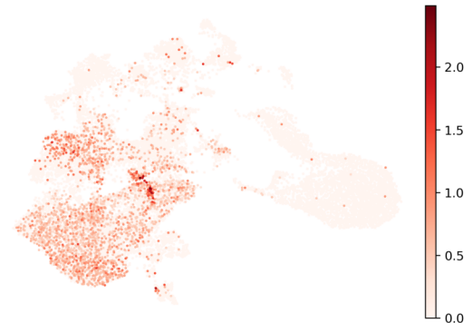
KIT
