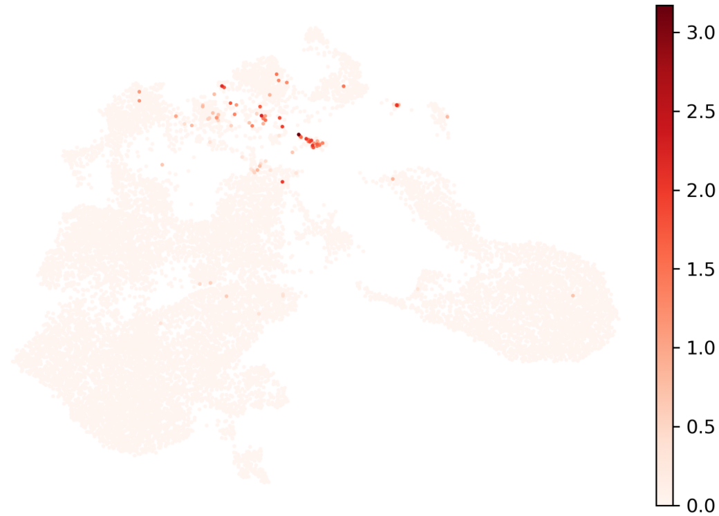
KRT19
