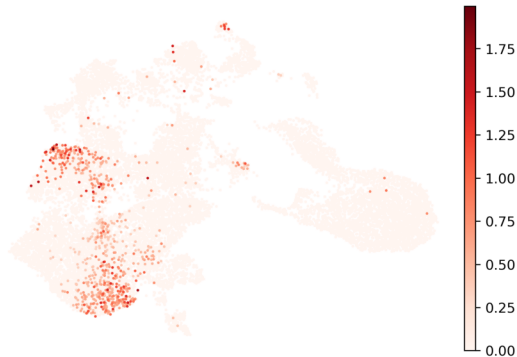
HLF
