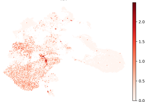
KIT
