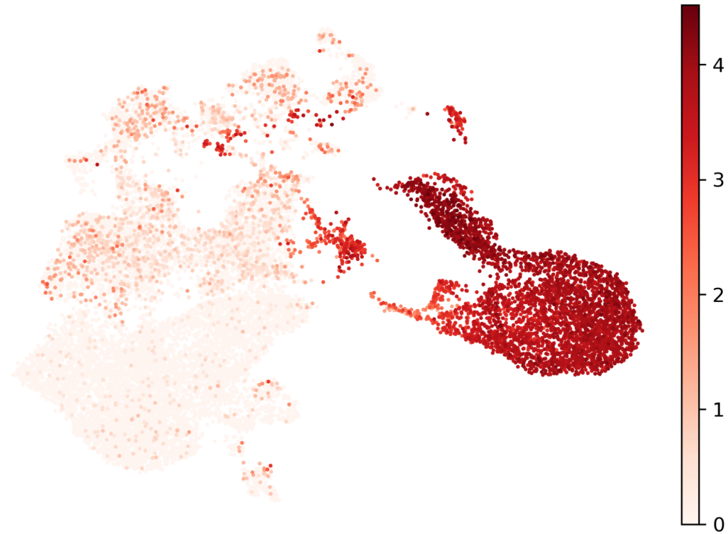
HBG1
