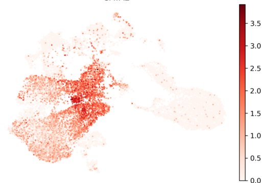
GATA2
