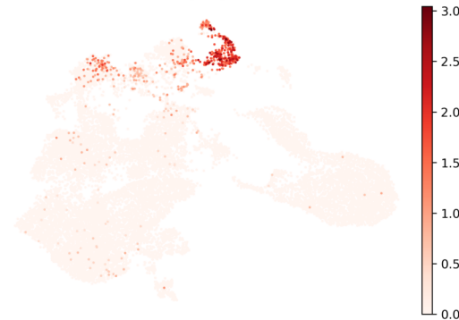
CDH5
