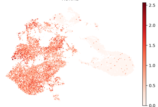
RUNX1
