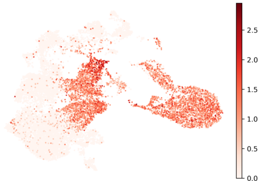
GATA1
