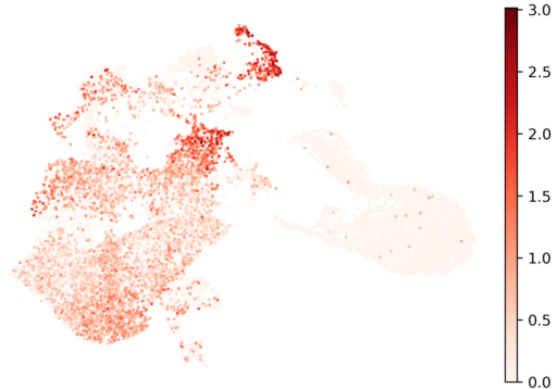
PECAM1
