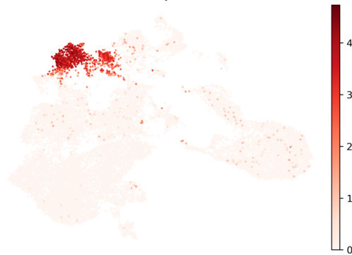
C1QC
