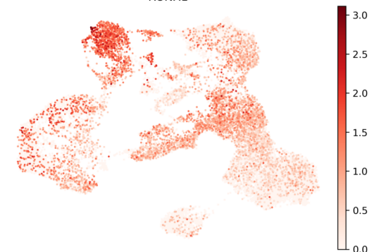
RUNX1
