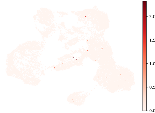
SOX2
