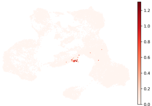
HLF
