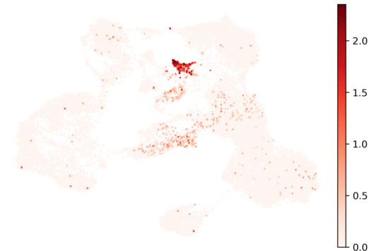
KIT
