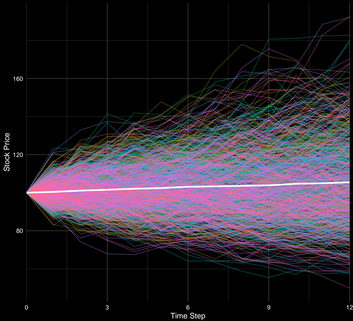
Monte Carlo Simulated Stock Price Paths with Average Path
