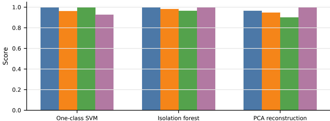
Baseline anomaly-detection performance on held-out test split
