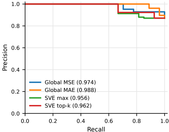
CNN-AE interpolated precision-recall curves
