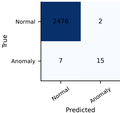
One-class SVM
