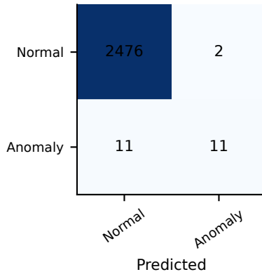
Isolation Forest
