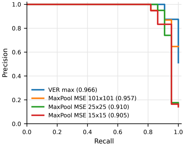
Broach dataset CNN-AE PR curves
