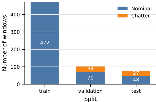
Frozen turning-dataset split
