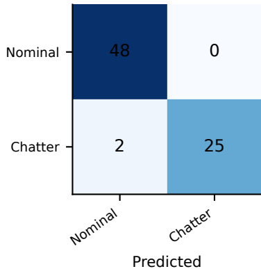
One-class SVM
