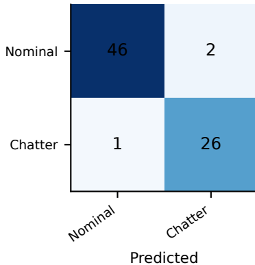
Isolation forest
